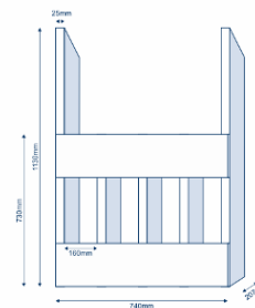
WOODEN CYLINDER RACK 4 X 10L CYLINDERS
